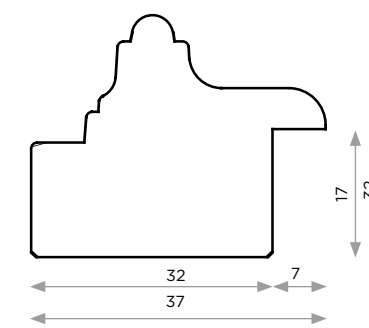
652 37mm x 32mm
